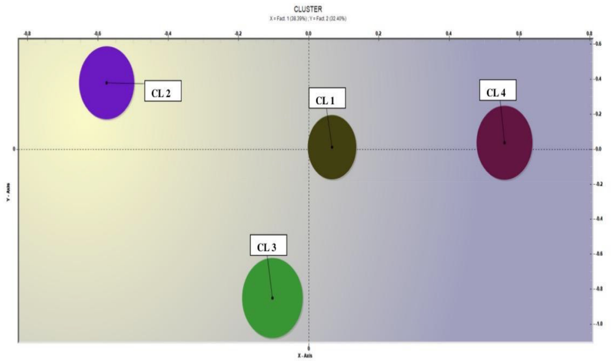
Figure 1. Factorial plan
